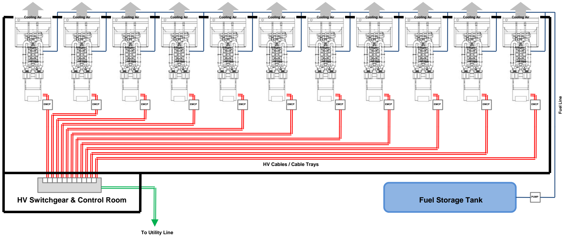
Example of 22MW / 27.5MVA @ 60Hz or 22MVA / 17.6MW @ 50Hz Power Plant
